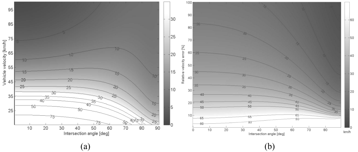
Figure 36: Accuracy of vehicle velocities estimated based on combining the two velocity components, (a) standard deviation \sigma_v^{a+c} as a function of target velocity v and the intersection angle \theta_v , \sigma_v^{a+c} is given in km/h; (b) Relative velocity error \sigma_v^{a+c}/v
