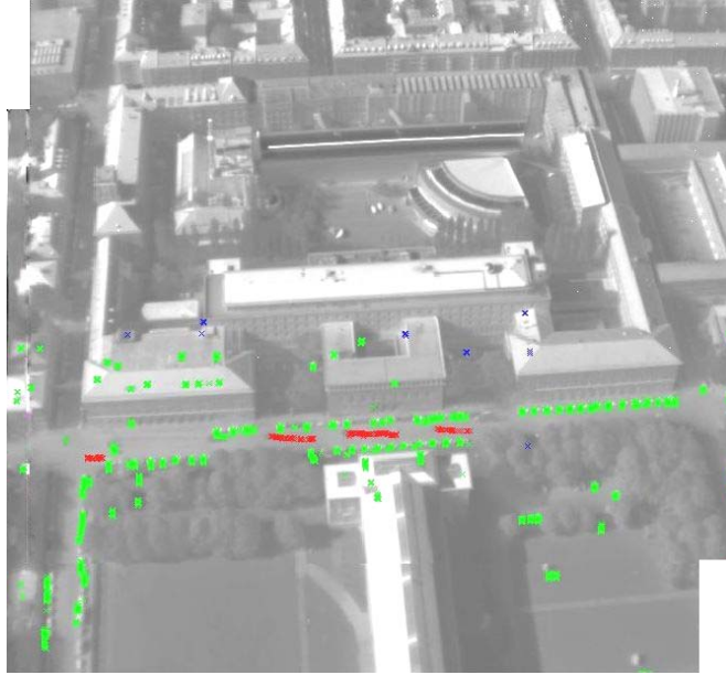
Figure 41: Video reference data for motion analysis displayed on a composite of two video frames, green: stationary vehicles, red: trajectories of moving vehicles
