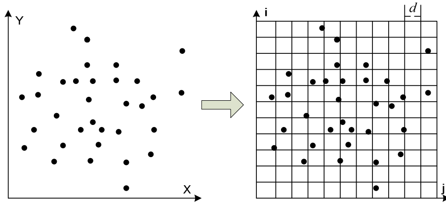
Figure 10: Schema of geo-tiling for LiDAR points indexing
