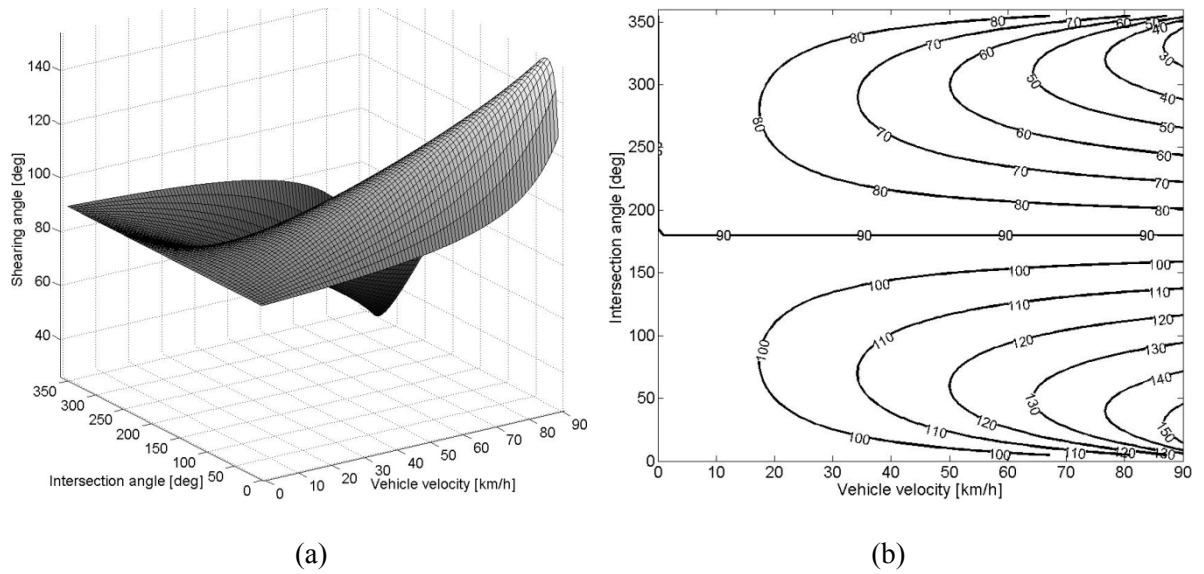
Figure 26: Shearing effect of a moving object in ALS data, (a) as function of \theta_v and v while v_L=100\text{km/h} , (b) contour plot of (a)
