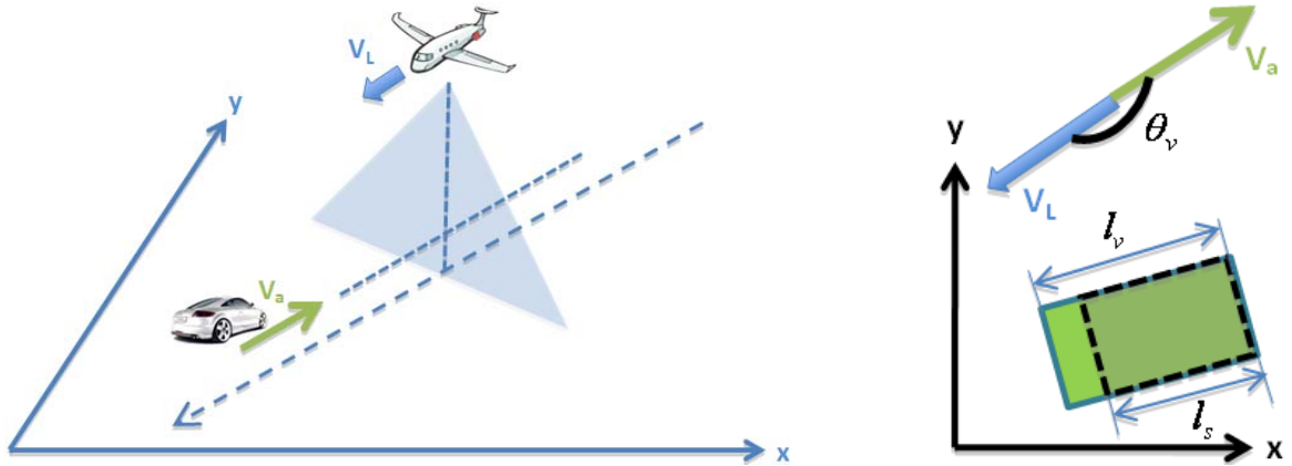
Figure 22: Along-track object motion
