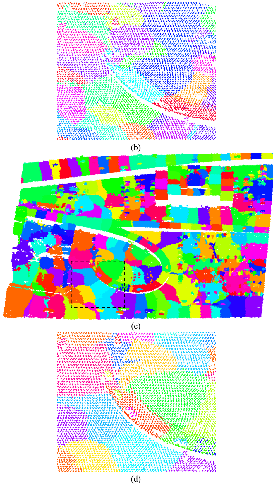
Figure 16: 3D segmentation of an ALS urban data by adaptive MS. (a) fixed-bandwidth (11m) MS, the number of objects = 592; the silhouette S = 0.343 ; (b) zoom into the box areas of (a); (c) variable-bandwidth MS. The number of object = 478; the silhouette S = 0.745 ; (d) zoom into the box areas of (c.)
