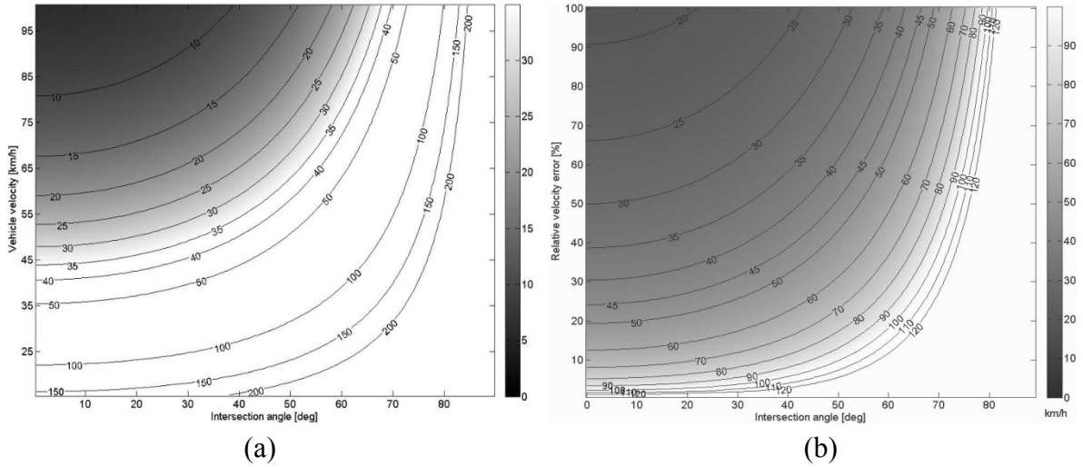
Figure 35: Accuracy of vehicle velocities estimated from the along-track stretching effect considering the error of the original aspect ratio Ar , (a) standard deviation \sigma_v^a as a function of target velocity v and the intersection angle \theta_v , \sigma_v^a is given in km/h, (b) Relative velocity error \sigma_v^a/v
