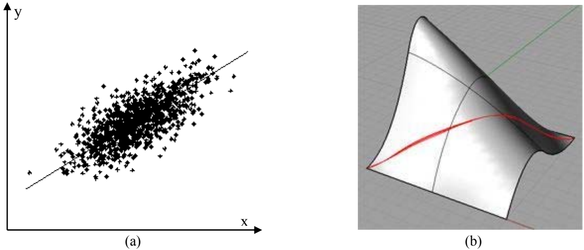
Figure 5: Comparison of PCA and PGA, (a) PCA in 2D feature space, (b) PGA in 2D manifold of feature space, red line indicates the principal geodesics
