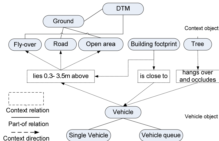
Figure 4: Local context-relations model in urban areas
