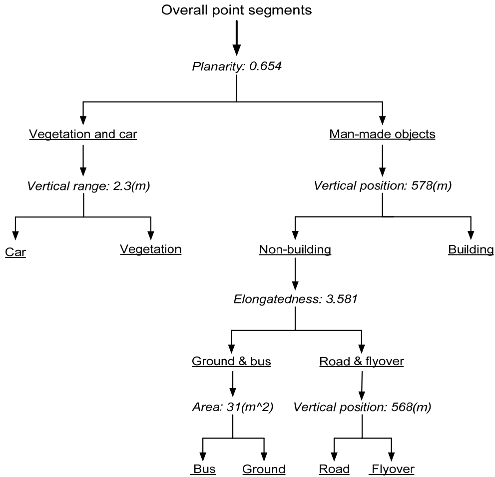
Figure 20: Classification tree for assigning the urban categories to segments in Figure 19
