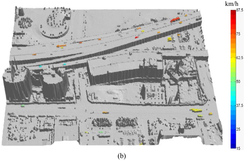
Figure 44: Vehicle motion analysis results for dataset Toronto II: (a) motion state classification, (b) velocity estimation
