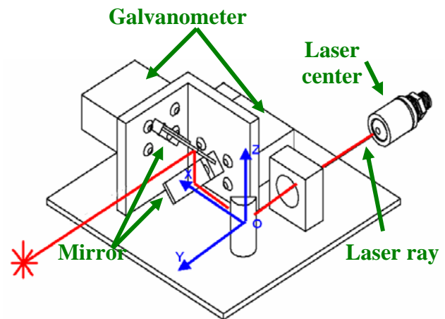
Figure 2. abstracted model of laser scanner. The red line represents the laser ray. The coordinate system (in blue) is the default coordinate system in the local scanning system.
