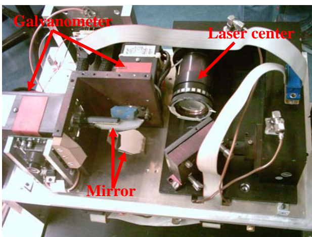
Figure 1. laser scanner with two galvanometers
