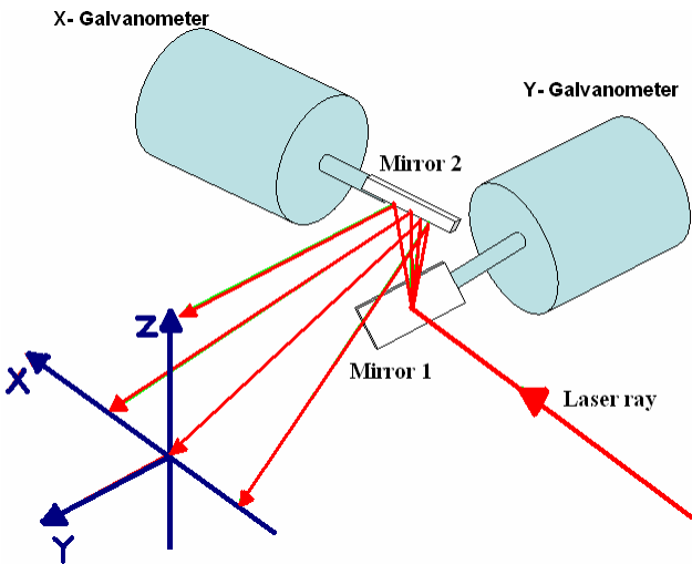
Figure 3. XY-Scanner
