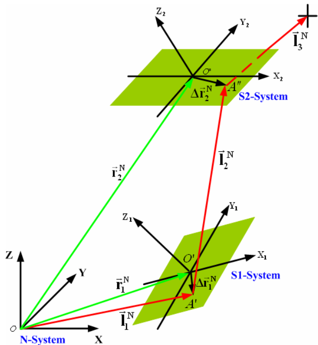
Figure 4. coordinate systems and vectors of the laser path
