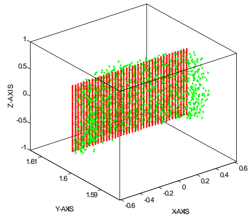
Figure 7. Measured data (in green) and their approximated plan (in red)
